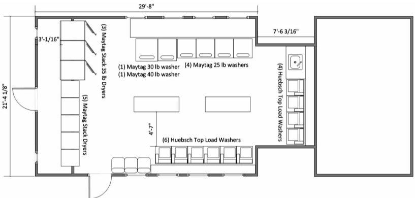
C-PEC's 3D renderings and floor plan layouts provide a realistic view of large capacity and energy efficient equipment options.
